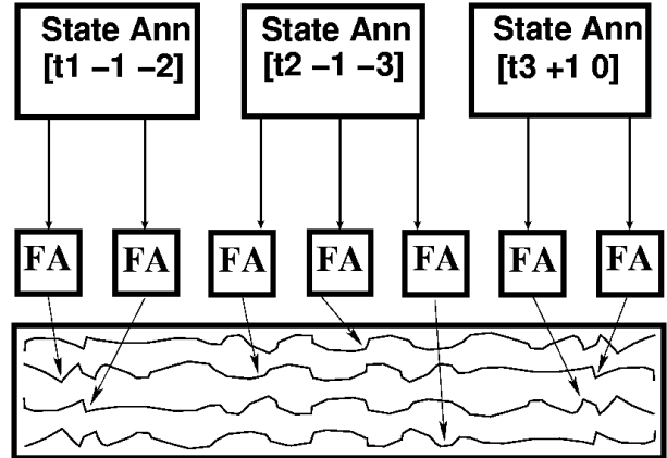
Figure 1. Annotation Scheme: This shows the three tiered approach to annotation. On the top tier, we see the /it-State Annotations, which have time values( t_1, t_2, t_3 ), trajectory assessments(-1, -1, +1) and state assessments(-2, -3, 0) which represent meanings as detailed in Table 2
